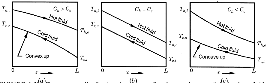
FIGURE 1.50 (a) Temperature distributions in a counterflow heat exchanger of single-phase fluids (no boiling or condensation). Here C_h = (\dot{m}c_p)_h is the heat capacity rate of the hot fluid, C_c is the heat capacity rate of the cold fluid, and specific heats c_p are treated as constant. The symbol T is used for temperature; the subscripts h and c denote hot and cold fluids, and subscripts i and o represent the inlet and outlet of the exchanger (Shah, 1981).
